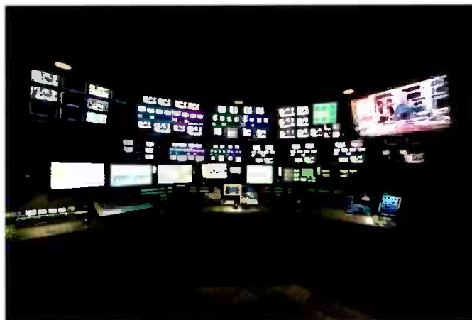
In the newly redesigned control room, Evertz monitors route the appropriate multiviewer outputs to one of 13 overhead displays, which are fed by a redundant analog Raritan KVM matrix.
